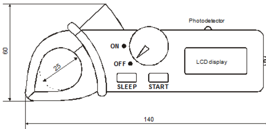
Figure 7. Dimensions of DC2-p portable locator pincers
