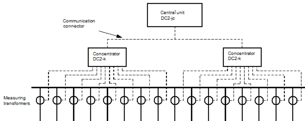
Figure 10. Diagram of basic measuring system for exemplary switching station in which 16 outgoing are measured.
