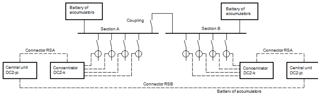
Figure 23. System DCtest-2 in two-section switching station
