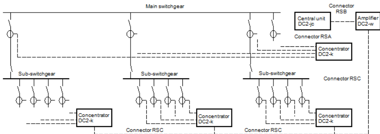
Figure 22. DCtest2 system in the main switchgear and sub-switchgears – variant 3.
