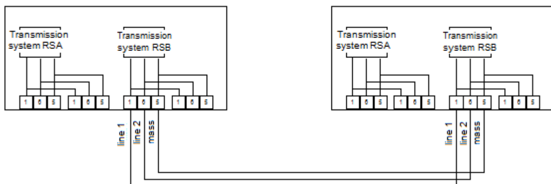
Figure 29. Exemplary diagram of connections between central units
