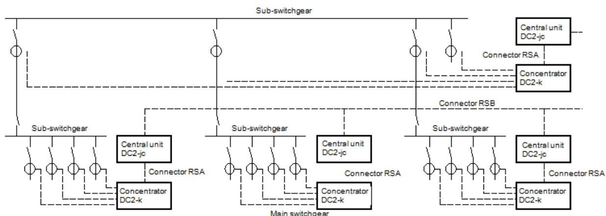
Figure 19. DCtest2 system in the main switchgear and sub-switchgears – variant 1.
