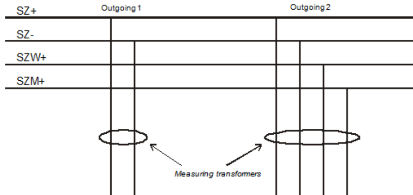
Figure 16. Connection of outgoing to buses of direct current switching station.
