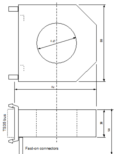
Figure 6. Dimensions of DC2-I43 measuring transformer
