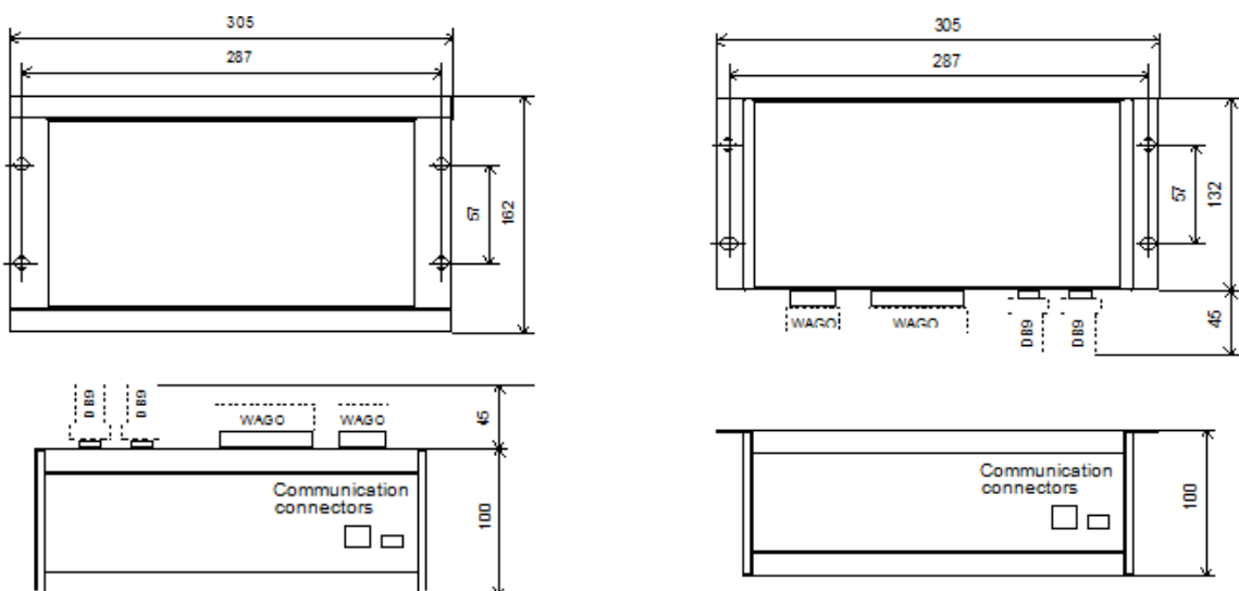
Figure 3. Dimensions of surface-mounted case
