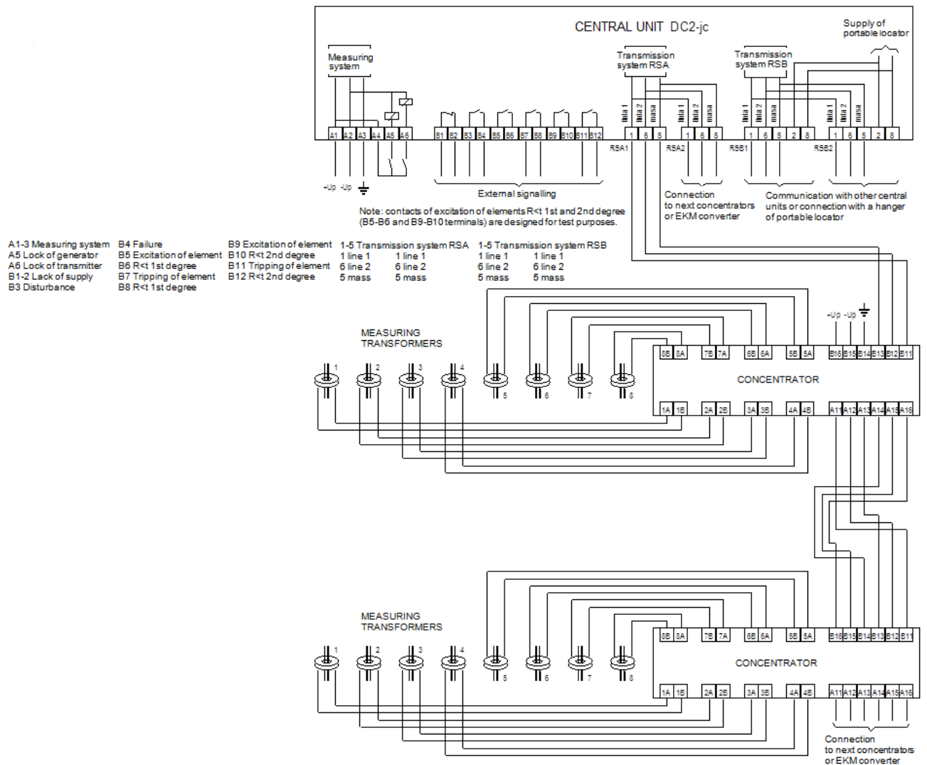
Figure 28. Exemplary diagram of connections between central unit, concentrators and measuring transformers.
