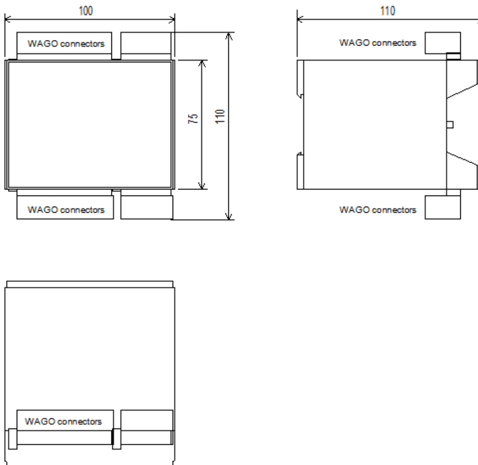
Figure 4. Dimensions of concentrator
