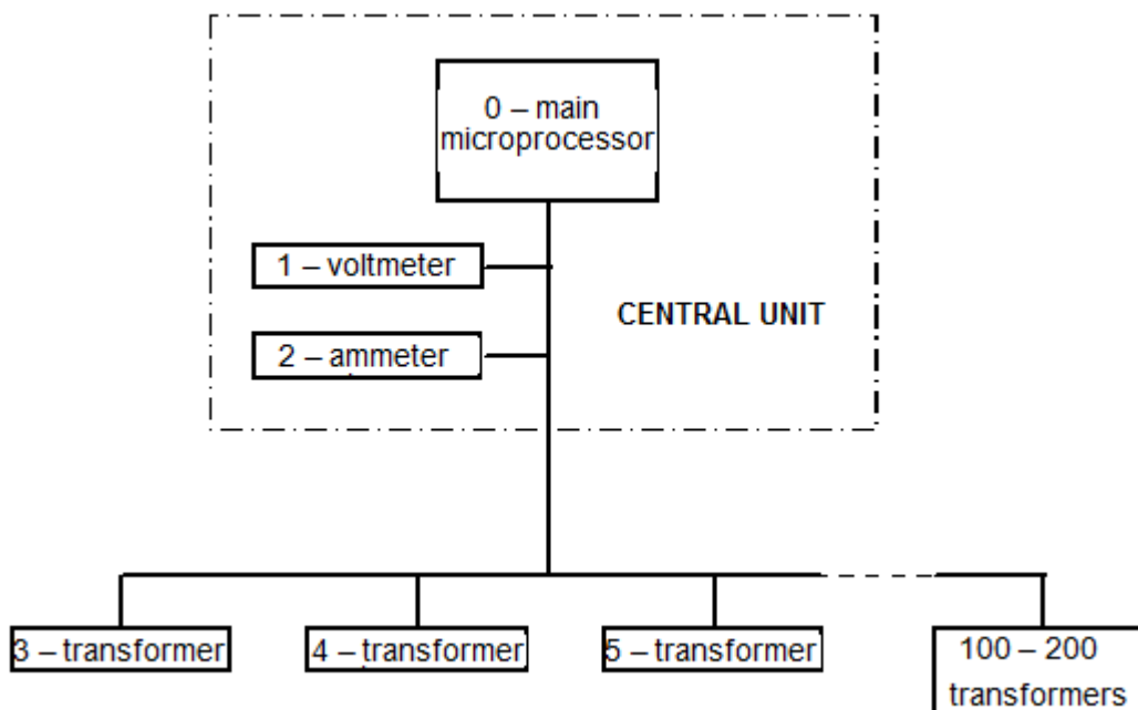
Figure 27. Principle of operation of RSA transmission system.
