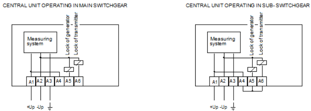
Figure 20. Diagram of locks of central units operating in one network
