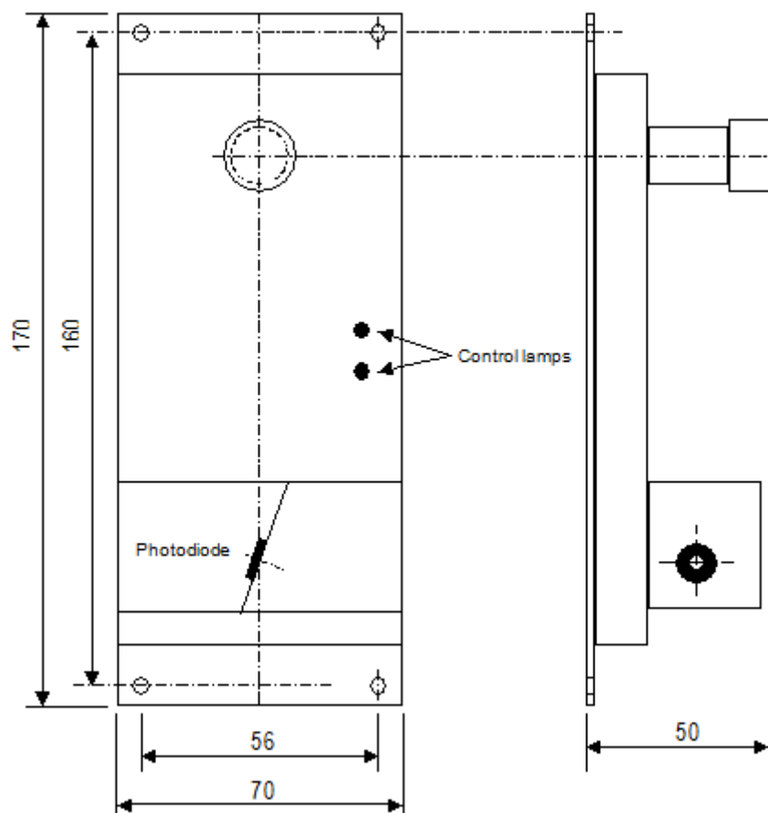
Figure 8. Dimensions of DC2-p portable locator hanger
