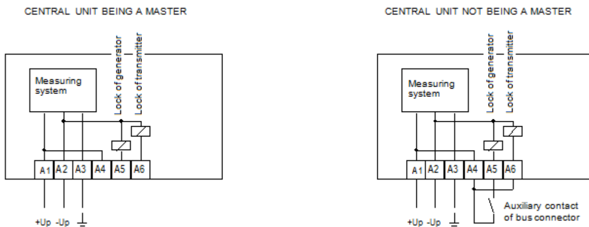
Figure 24. Diagram of locks of central units working in one network
