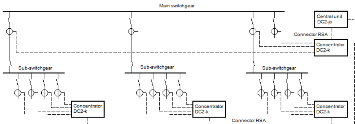
Figure 21. DCtest2 system in the main switchgear and sub-switchgears – variant 2.
