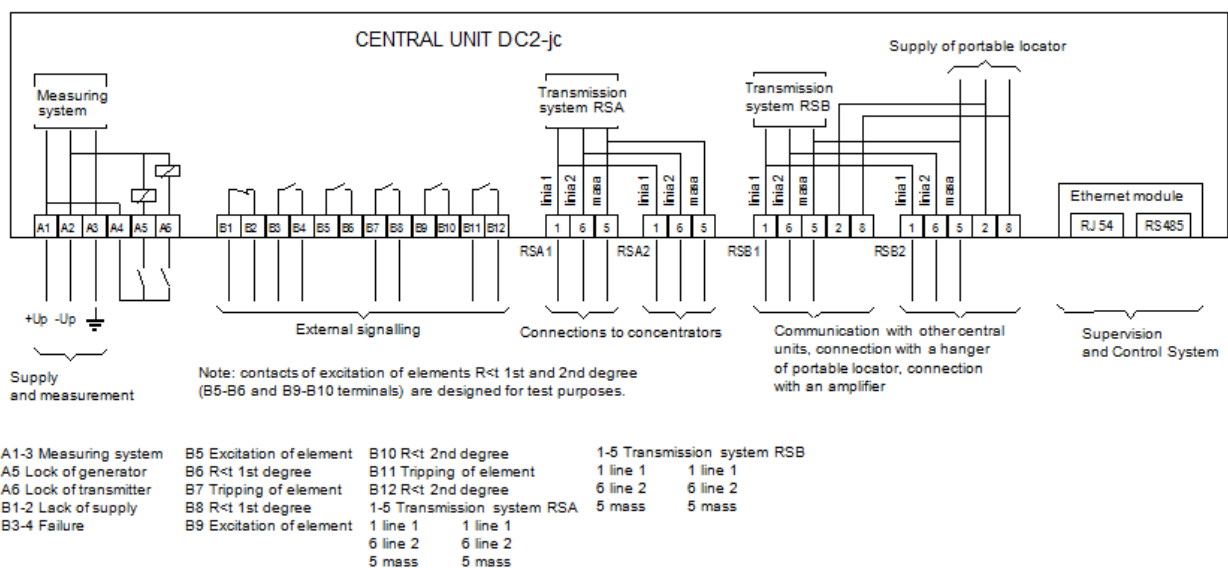
Figure 25. Diagram of external connections of central unit.
