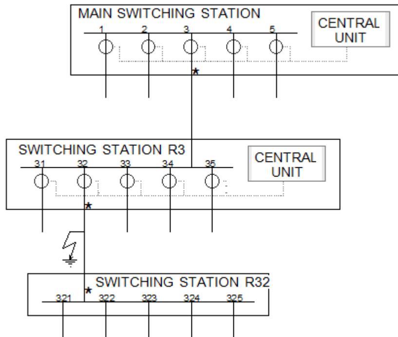
Figure 37. Location of earth fault in direct current network.
