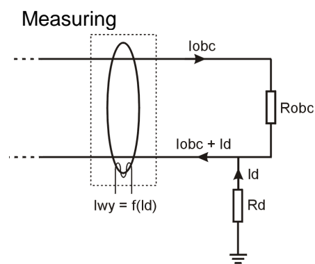
Figure15. Principle of operation of stationary measuring transformer.
