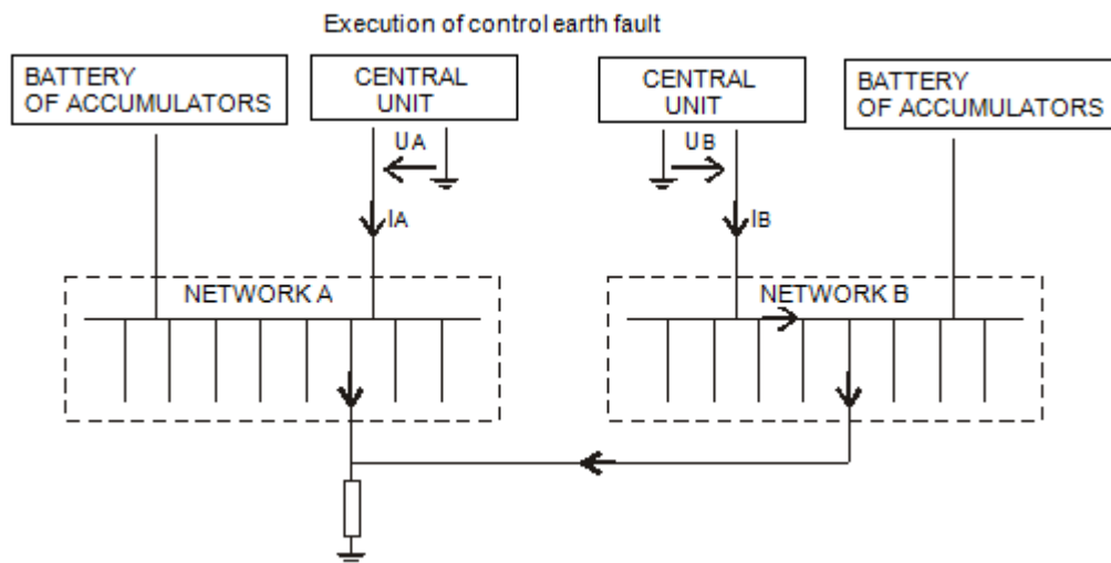
Figure 39. Methods of detection and location of connections between batteries.
