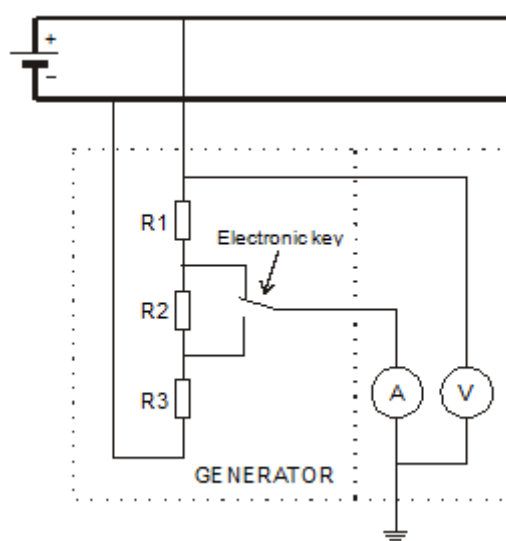
Figure 11. Generator operation concept and voltmeter and ammeter connection.
