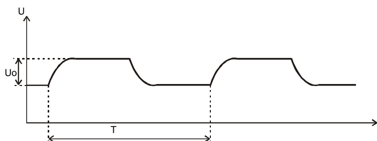
Figure 12. Shape of output generator pattern.
