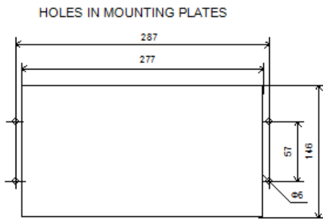
Figure 2. Dimensions of 14-inch flush-mounted case
