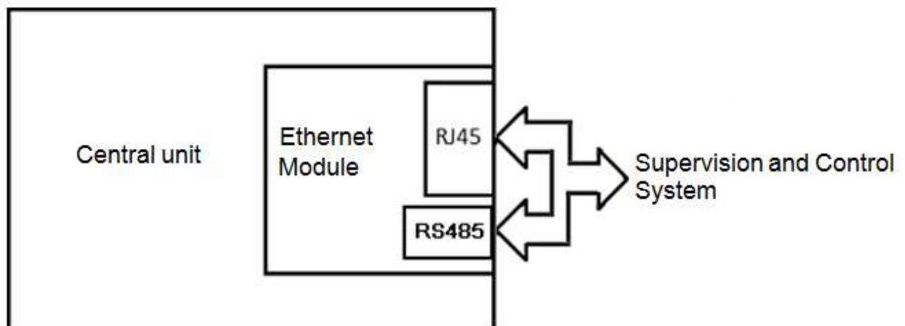
Figure 30. Ethernet Module built inside Central Unit
