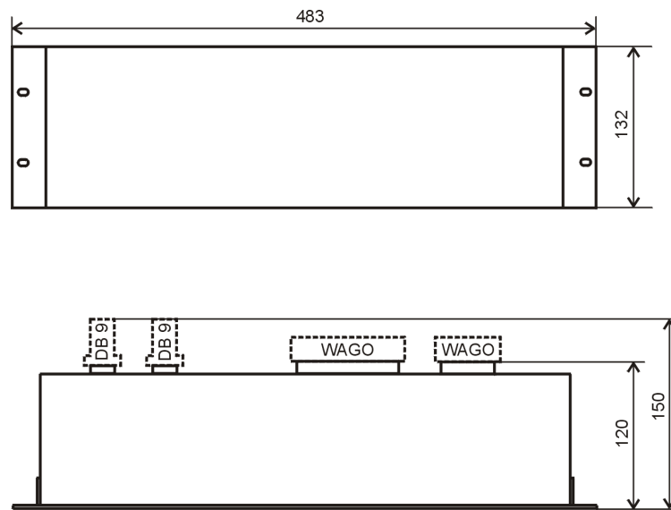
Figure 1. Dimensions of 19-inch flush-mounted case.
