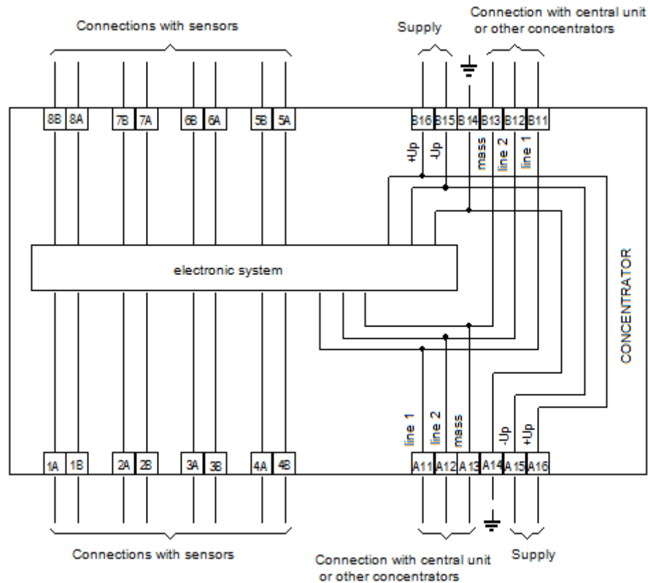
Figure 26. Diagram of external connections of concentrator.
